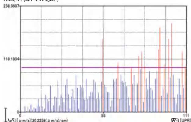
Velocity分析[圆度<Round_15>]
